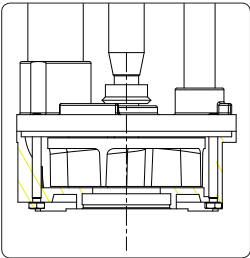
Version V: with bottom for extension tube.
