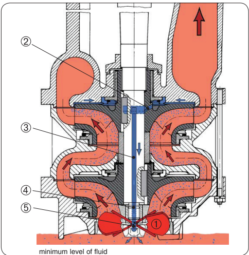
Model PSL centrifugal slurr pumps for fluids containing large amounts of trapped air
